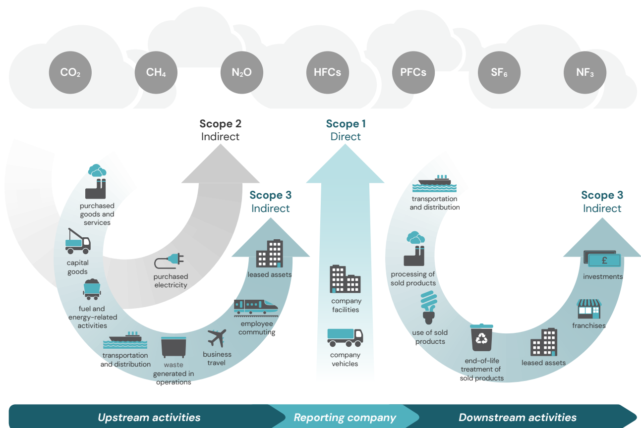
An illustration of the Scopes and Categories that make up a carbon footprint. Source: The GHG Protocol.
